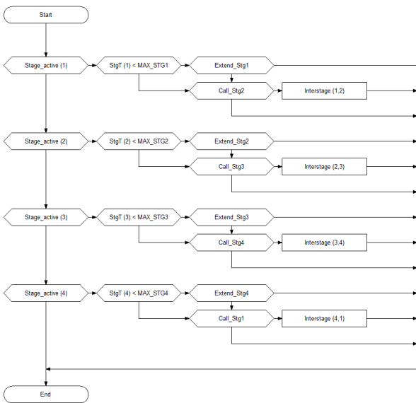
Figure 9 VISSIM algorithm
