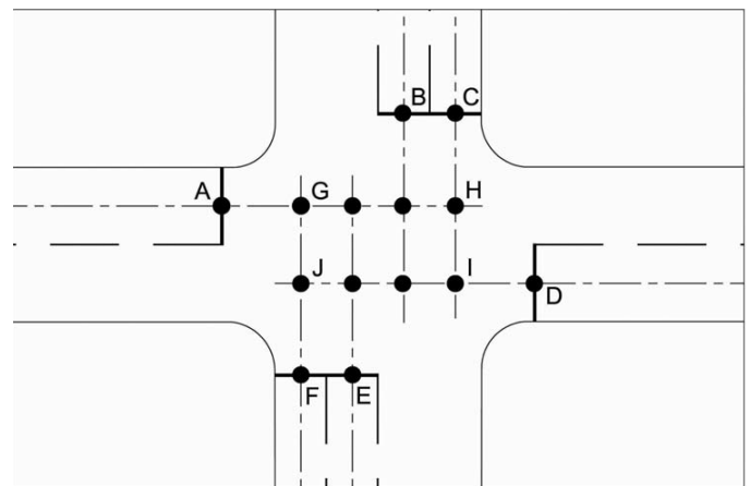
Figure 2 Conflict points (4-legged intersection)
