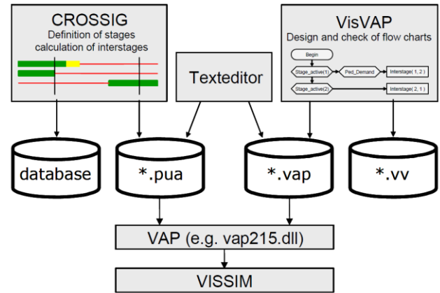
Figure 8 VisVAP flowchart [9]
