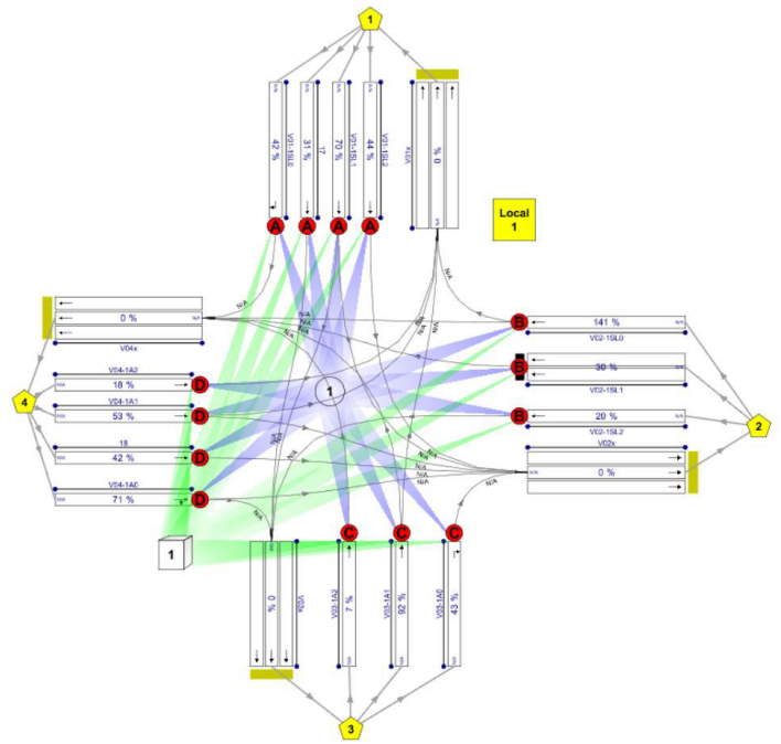
Figure 1 Intersection Network Diagram - TRANSYT
