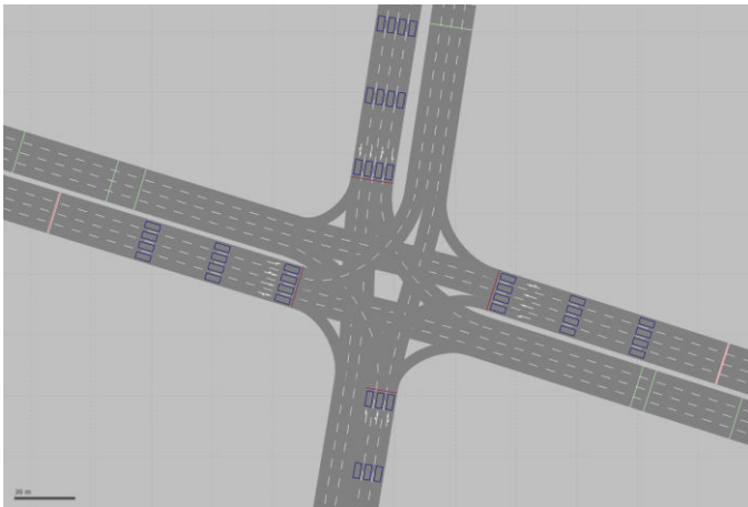
Figure 7 VISSIM traffic model
