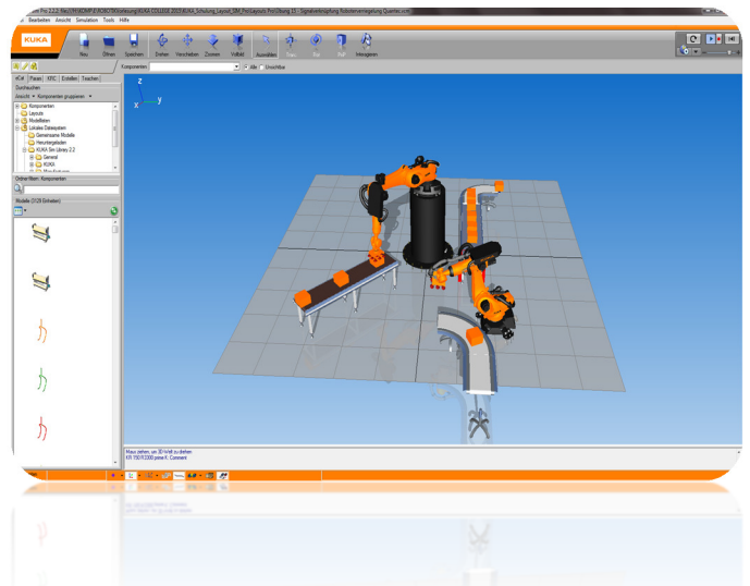
Figure 3. KUKA Sim Pro Ver.2.2 (own screenshot)
