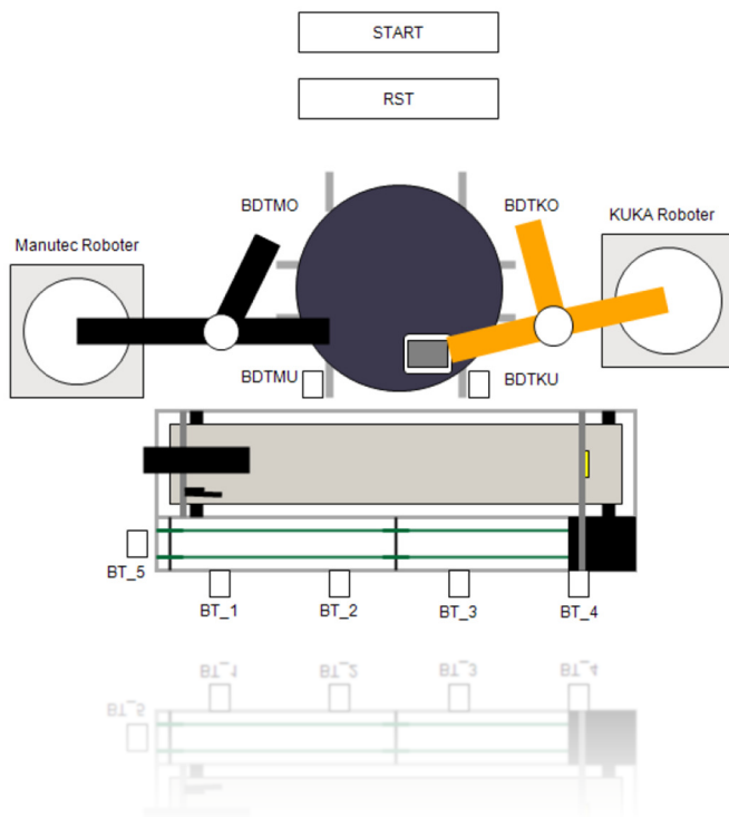
Figure 4. CODESYS Visualisation in RFH laboratory (own screenshot)
