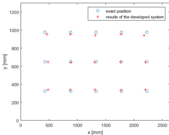
Figure 8. Results of static testing: blue circles denote actual positions measured by the referent localization system and red crosses represent the output of the developed system.
