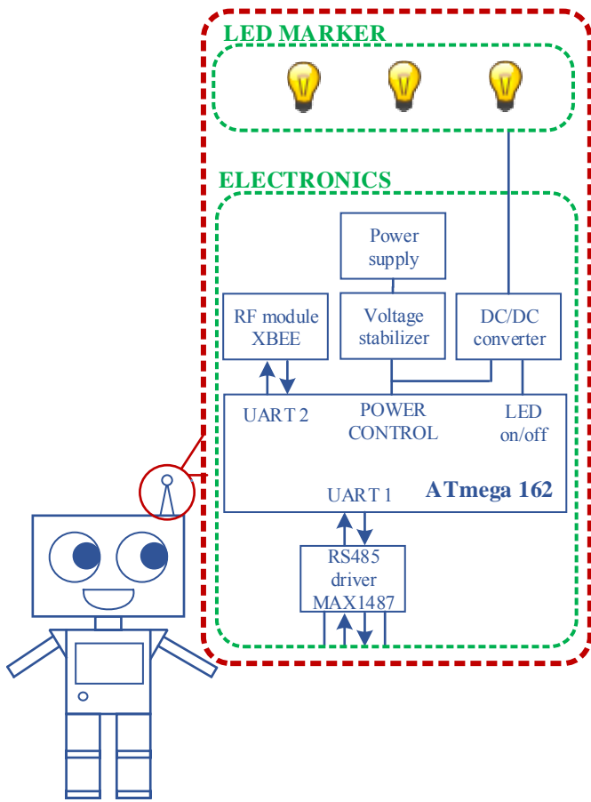
Figure 6. Structure of the active LED beacon.
