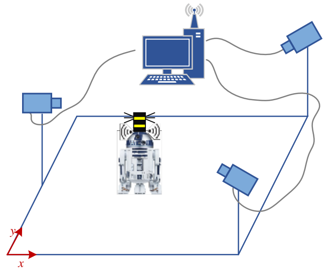
Figure 1. Design of the localization system.
