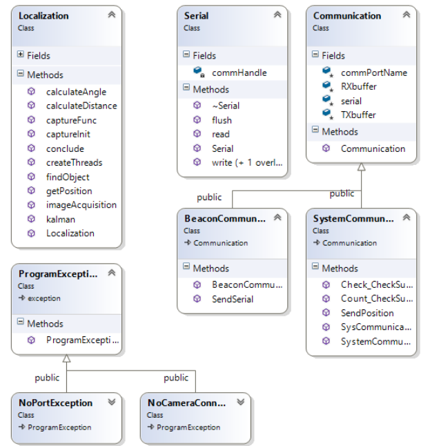
Figure 5. UML diagram.
