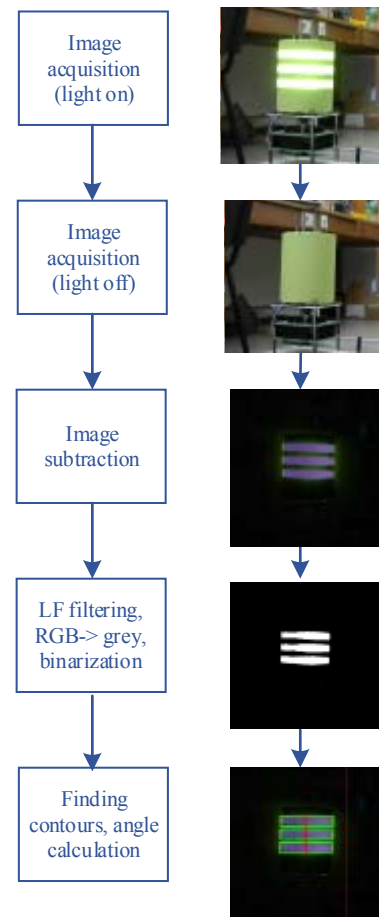
Figure 3. Image processing algorithm.
