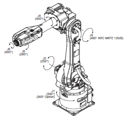
Fig.2. Isometric view of the ARC Mate 120iB
