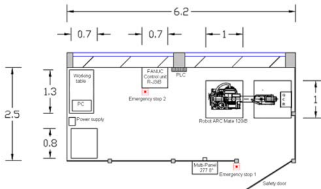
Fig. 1. Top view on the robot cell
