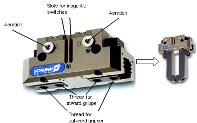
Fig.5. Pneumatic 2-Finger Parallel Gripper PGN-plus 80
