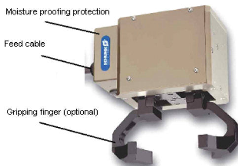
Fig.3. Electric 2-Finger Parallel Gripper PG 70
