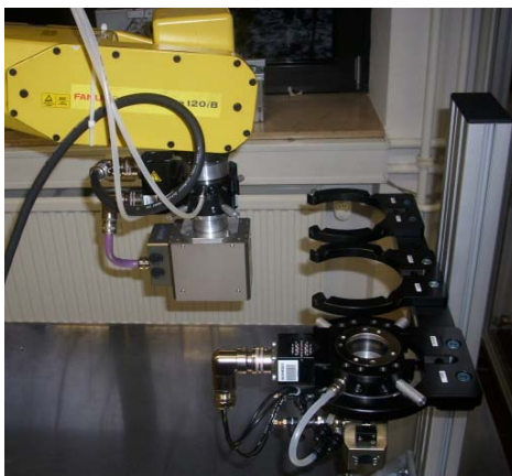
Fig. 17. Gripper-Change-System in operation
