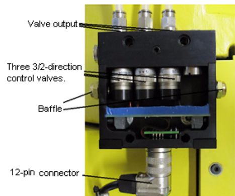
Fig. 10. Connected ganged valve
