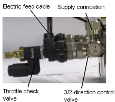
Fig. 8. Realized pneumatic actuation device
