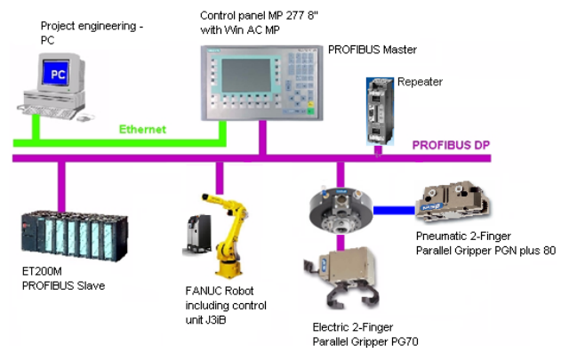
Fig.13. Communication system
