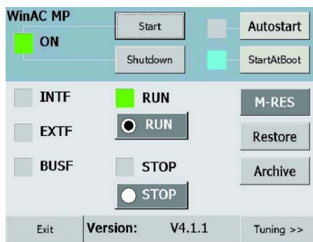
Fig. 16. Finished GUI
